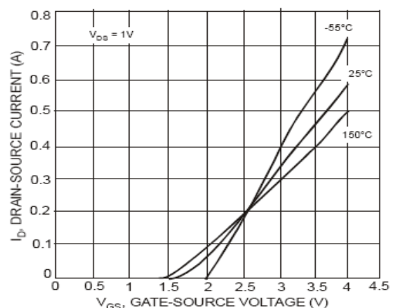
Fig. 2 Transfer Characteristics
